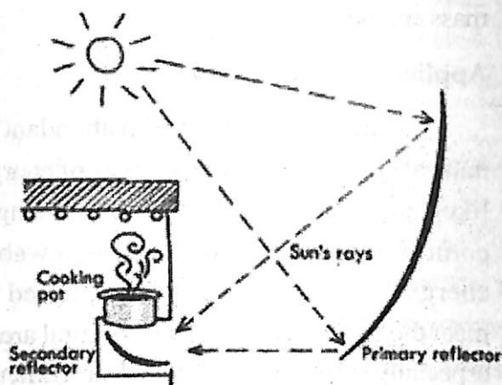
Fig: schematic of solar cooker
