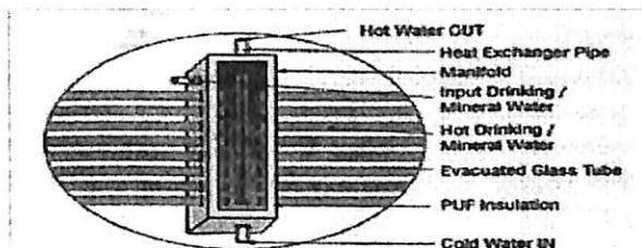
Fig : Pressurized Solar Heater
